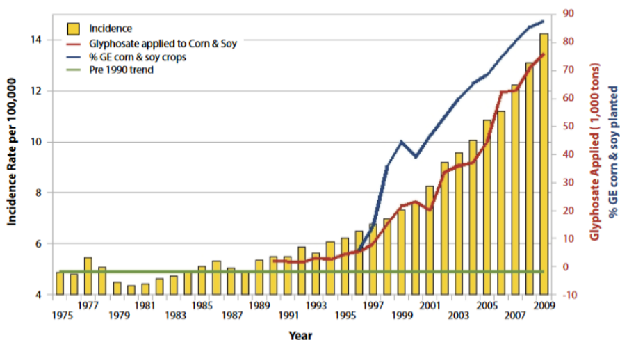
Figure 3. Thyroid cancer incidence rate plotted against glyphosate applied to U.S. corn & soy crops ( R=0.988 , p<7.612e-09 ) along with %GE corn & soy crops ( R=0.9377 , p<2.152e-05 ). Sources: USDA:NASS; SEER. (Figure courtesy of Nancy Swanson).
